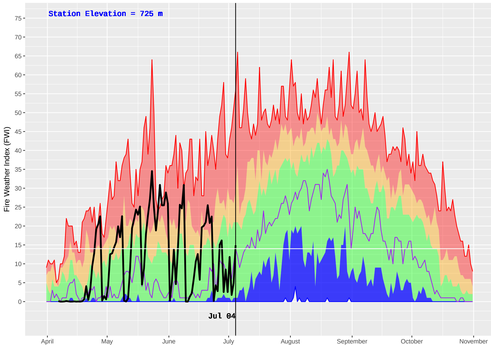
PENDOREILLE (402) : Historical (1986–2016) and Current (2018) Noon Fire Weather Index (FWI)
